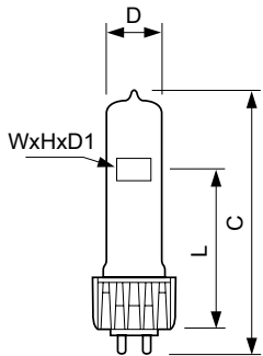
7007/LL 575W Heat Sink 230V
