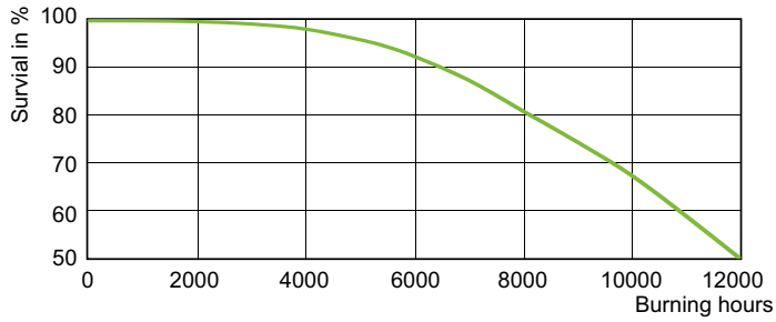
CDM-R 70W Life Expectancy /830 PAR30L
