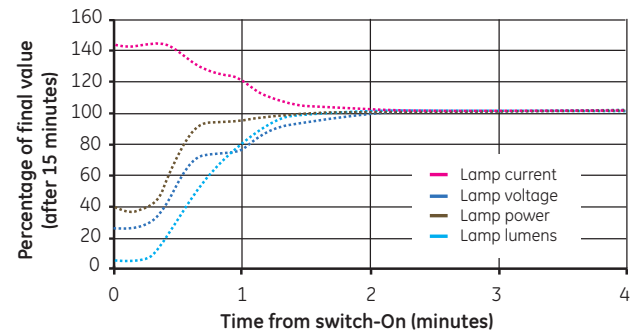
CMH MR16 35W typical warm-up characteristic
